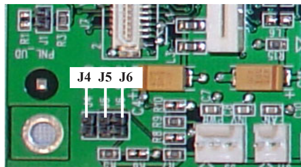
JUMPERS LOCATION
